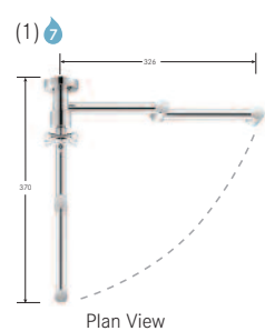
Plan View
